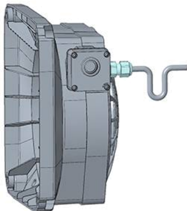
Fig. 1: Cable routing in U-shaped loop
